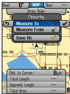
Fig 41. Measuring Menu-Basic Options
